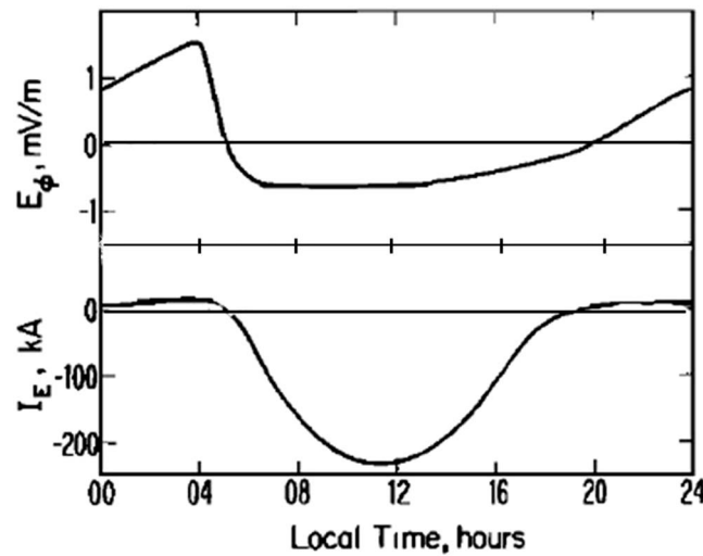
Figure 3. From Blanc and Richmond [1980].
