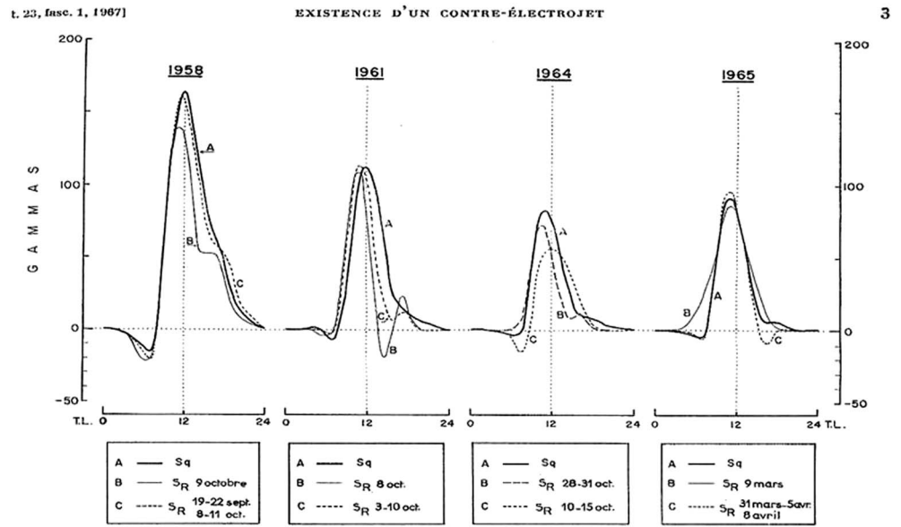
Figure 2. From Gouin and Mayaud [1967]. S_q and S_R curves of the H component at Adis Abeba, during equinoxes, for an individual day or for a series of individual days of the same season corrected for the noncyclic variation.
