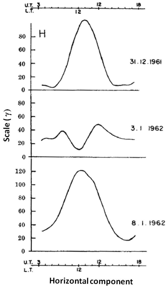
Figure 1. Extreme phase of the phenomenon showing the reversal in the direction of the H component daily variation on 3 January 1962 [after Gouin, 1962].
